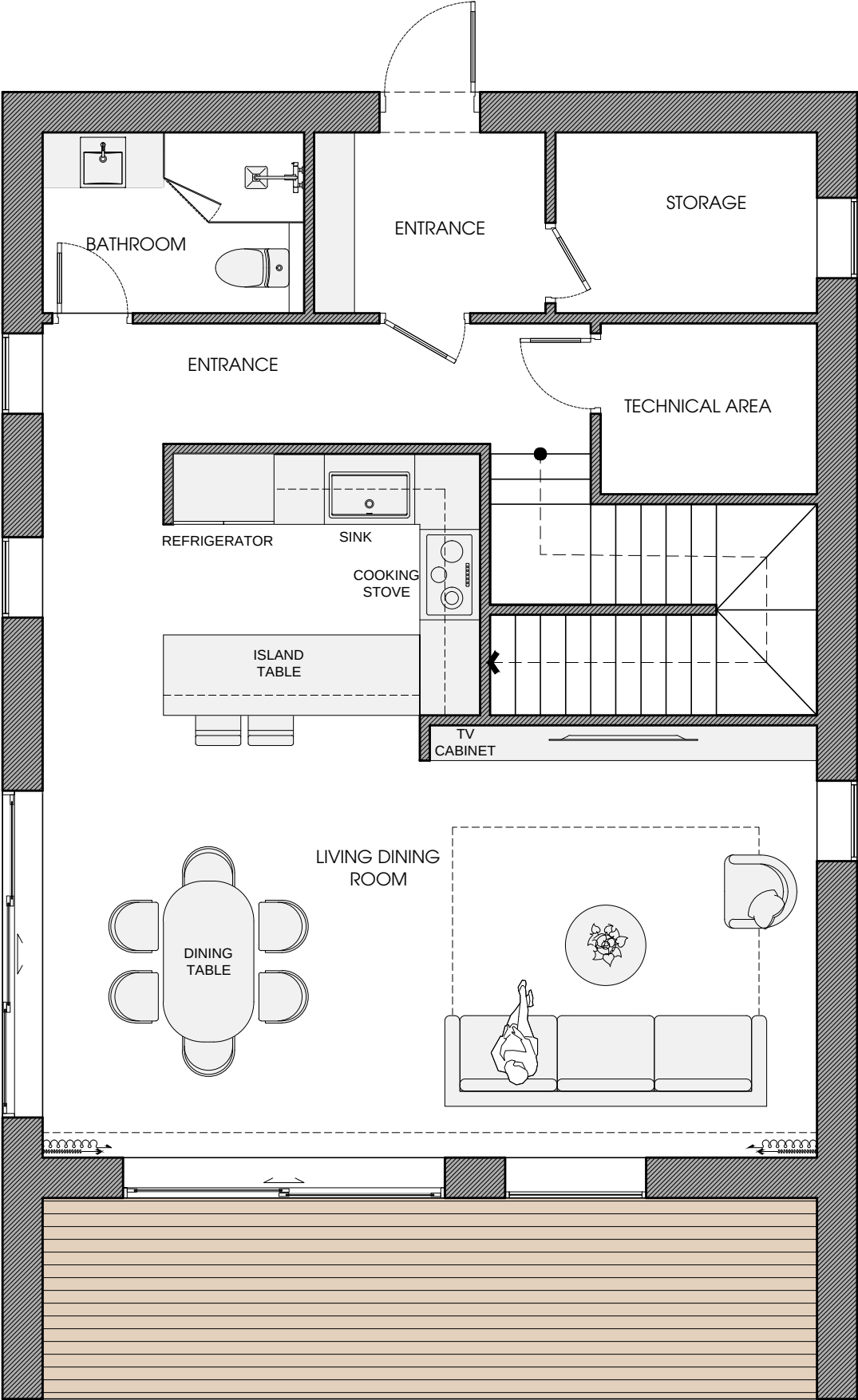
GROUND FLOOR
